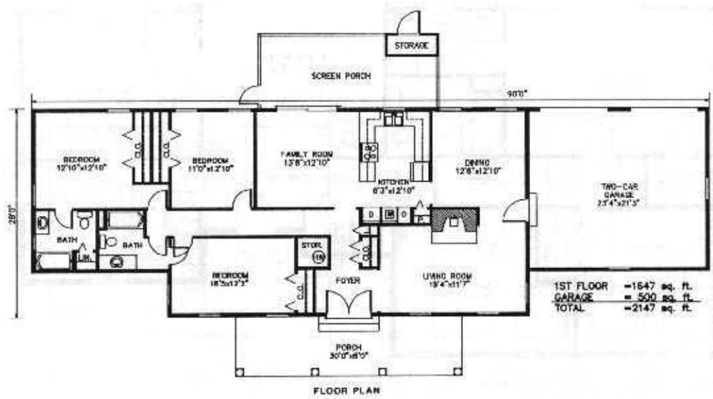
FLOOR PLAN
