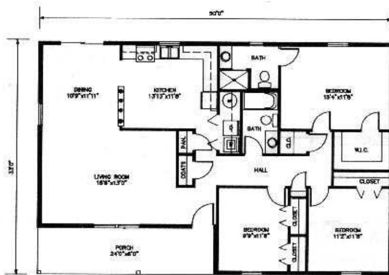
FLOOR PLAN
