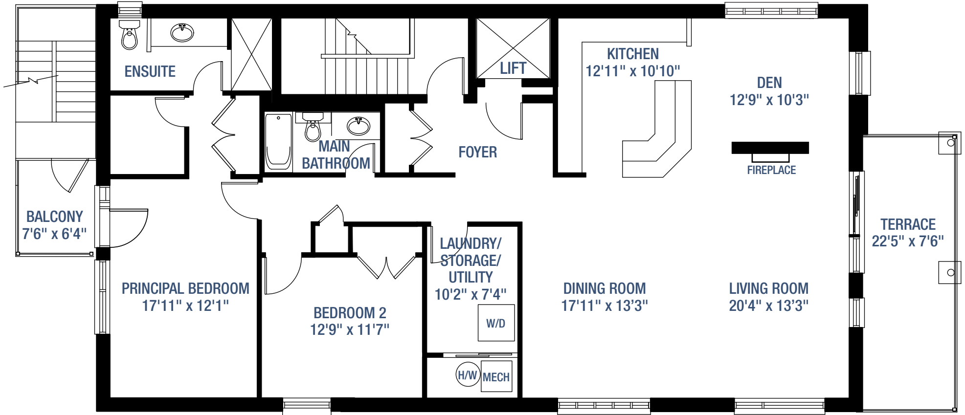
TYPICAL FLOOR PLAN 570 & 572 ATHLONE PRIVATE
